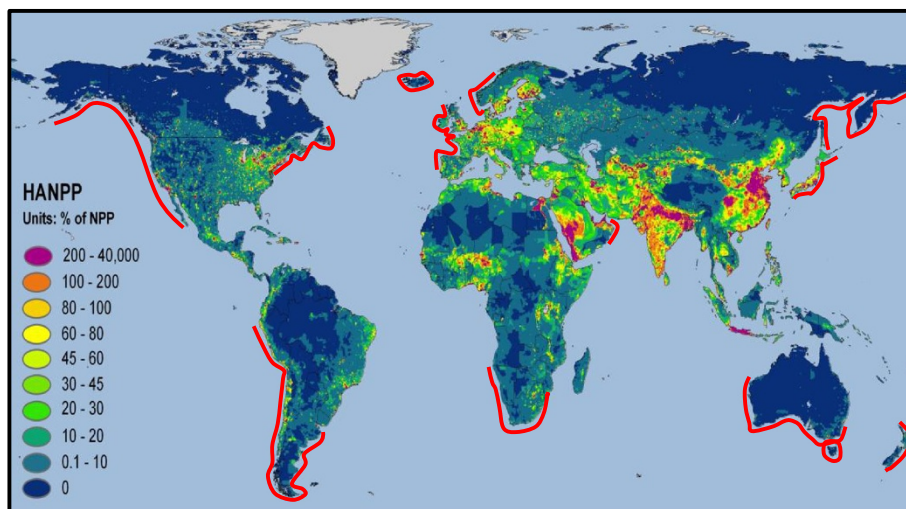
Figure 1 Natural distribution of shallow water macroalgae (red line) indicating coastal areas with the potential to culture macroalgae for biogas, and human appropriation of net primary production as a percentage of local net primary productivity (NPP) (NASA 2004 [30]). Redrawn from Santelices (2007) [31] and NASA Earth Observatory 2004.
