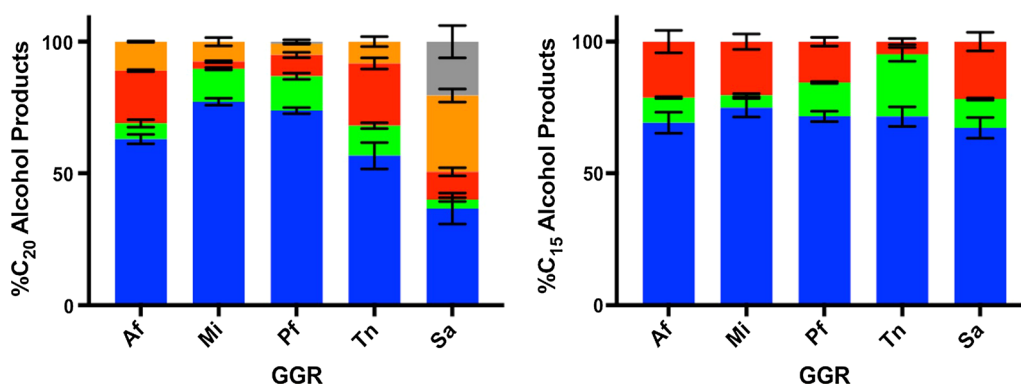
Fig. 4 Endpoint activity profiles for GGR reduction of either GGOH (left) or FOH (right) incubated under standard assay conditions for 1 h. Product distributions are represented as relative percentages of unreduced substrate (blue), H 2 -GGOH or H 2 -FOH (green), H 4 -GGOH or H 4 -FOH (red), H 6 -GGOH or H 6 -FOH (orange), and H 8 -GGOH (gray)
